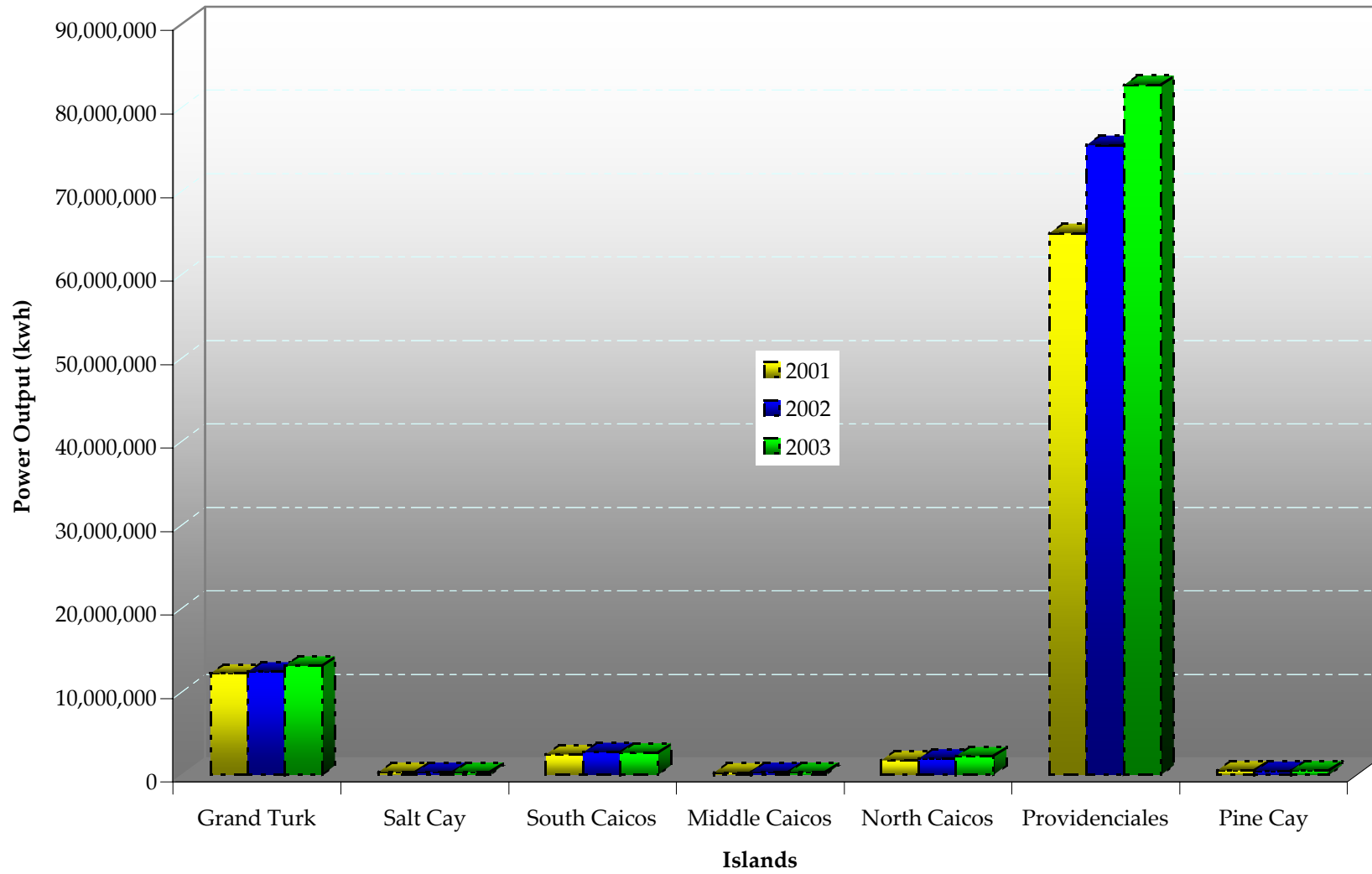
Electrical Power Output 2001 - 2003
